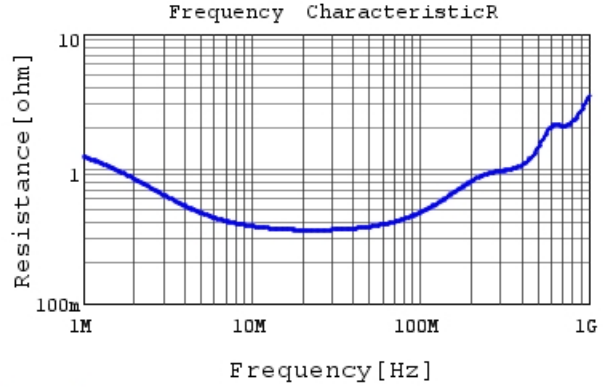
DE6E3KJ472MB4B R DC0V, 20degC
