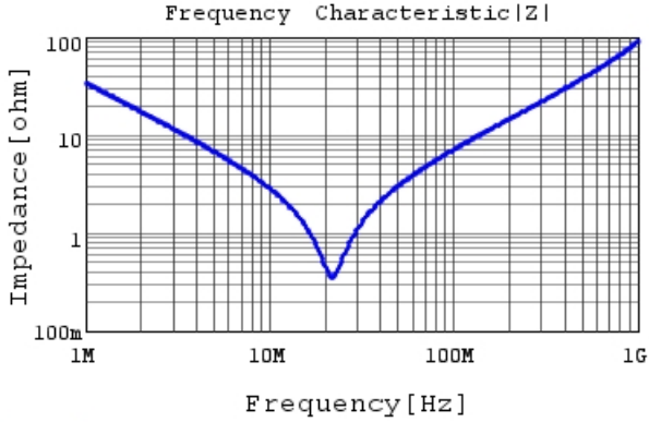
DE6E3KJ472MB4B |Z| DC0V, 20degC
