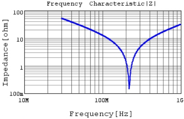
RCE5C2E101J1K1H03B |Z| DC0V, 25degC
