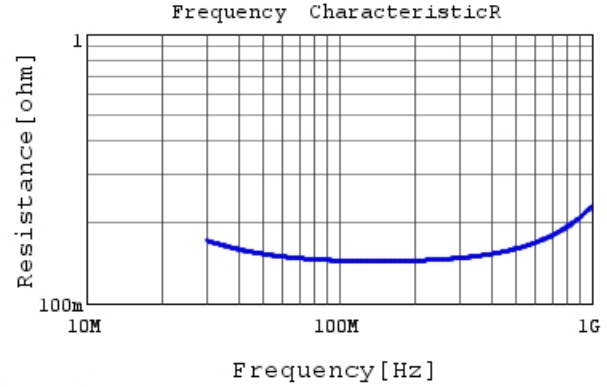
RCE5C2E101J1K1H03B R DC0V, 25degC
