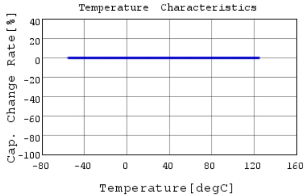
RCE5C2E102J1K1H03B C-Temp. capchange, DC0V,
