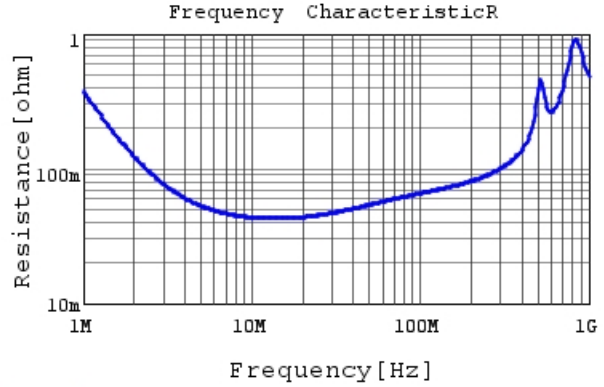
RCE5C2E102J1K1H03B R DC0V, 25degC
