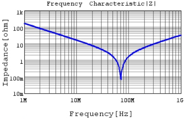
RCE5C2E102J1K1H03B |Z| DC0V, 25degC
