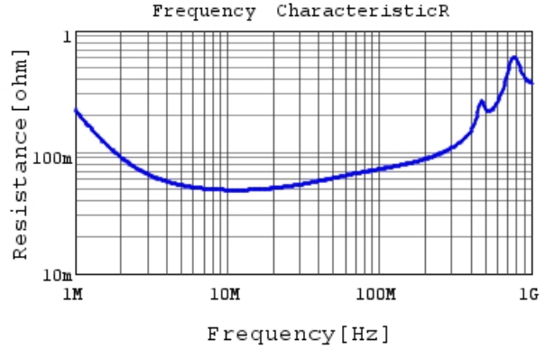
RCE5C2E152J1K1H03B R DC0V, 25degC
