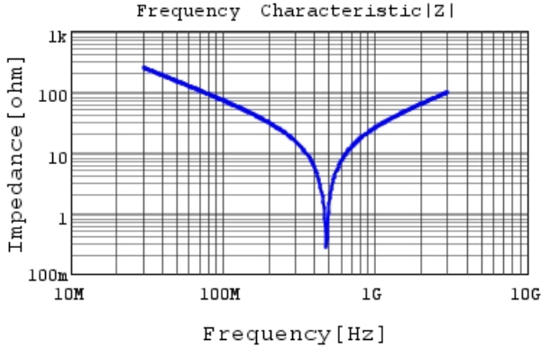
RCE5C2E220J1K1H03B |Z| DC0V, 25degC
