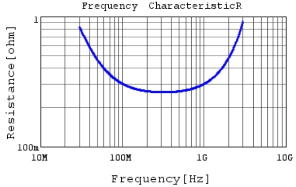
RCE5C2E220J1K1H03B R DC0V, 25degC
