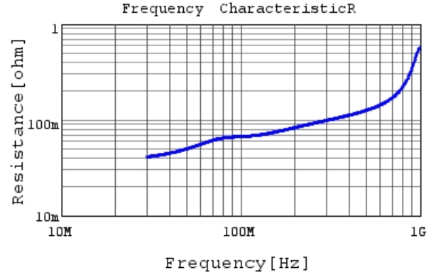
RCE5C2E331J1K1H03B R DCOV,25degC
