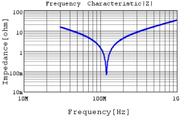
RCE5C2E331J1K1H03B |Z| DCOV,25degC
