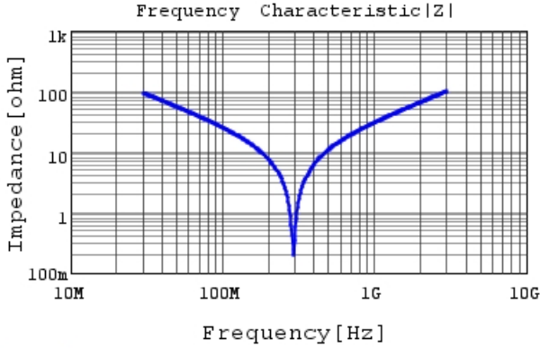
RCE5C2E560J1K1H03B |Z| DC0V, 25degC
