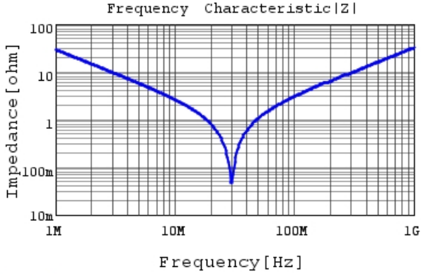
RCE5C2E562J1K1H03B |Z| DC0V, 25degC
