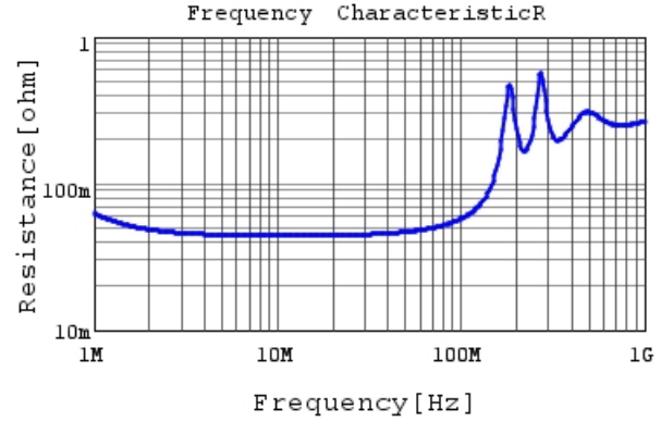
RCE5C2E562J1K1H03B R DC0V, 25degC
