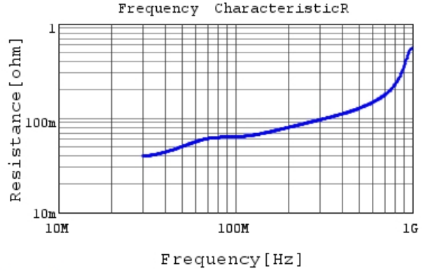
RCE5C2J331J1K1H03B R DC0V, 25degC
