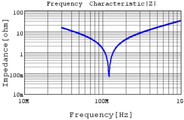
RCE5C2J331J1K1H03B |Z| DC0V, 25degC
