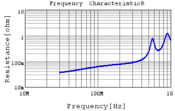
RCE5C2J681J1K1H03B R DC0V, 25degC
