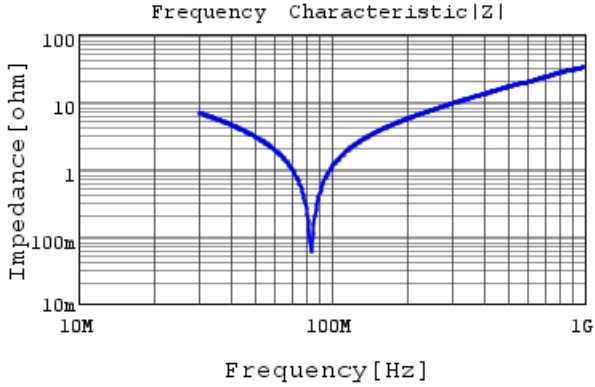
RCE5C2J681J1K1H03B |Z| DC0V, 25degC
