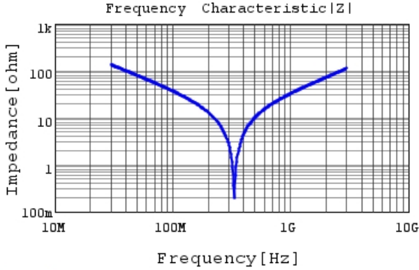
RCE5C3A390J2M1H03A |Z| DC0V, 25degC
