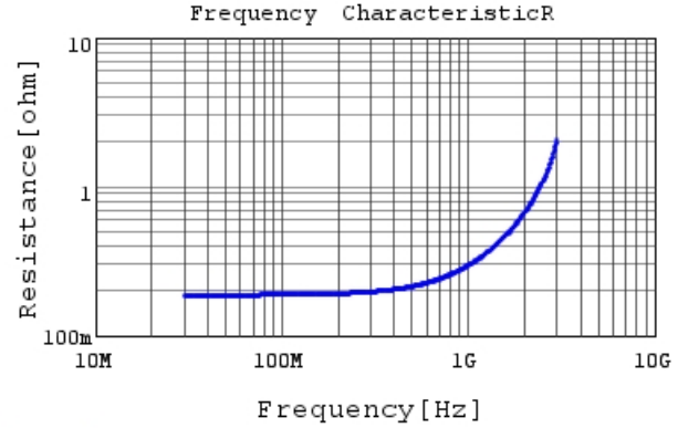
RCE5C3A390J2M1H03A R DC0V, 25degC
