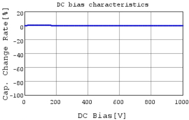
RCE5C3A390J2M1H03A C-DC bias capchange, 25.0
