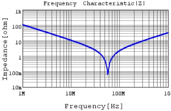
RDE5C2E152J1K1H03B |Z| DC0V, 25degC
