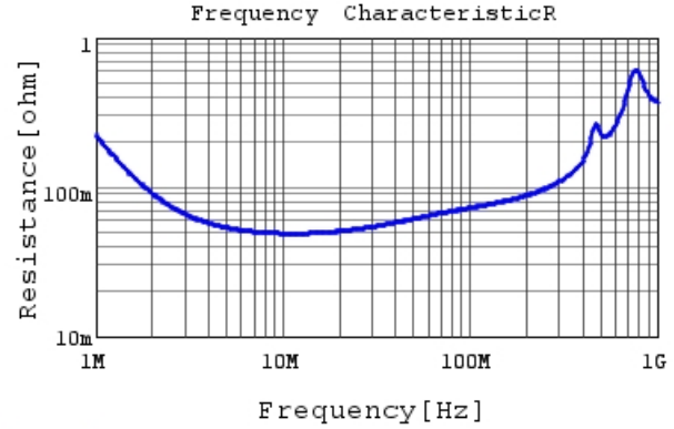
RDE5C2E152J1K1H03B R DC0V, 25degC
