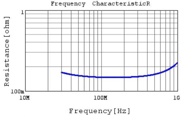
RDE5C2J101J1K1H03B R DC0V, 25degC
