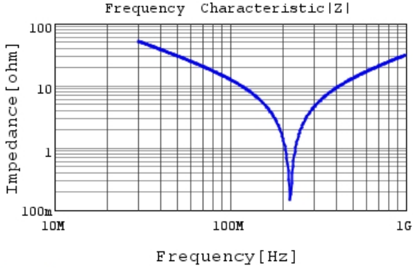
RDE5C2J101J1K1H03B |Z| DC0V, 25degC
