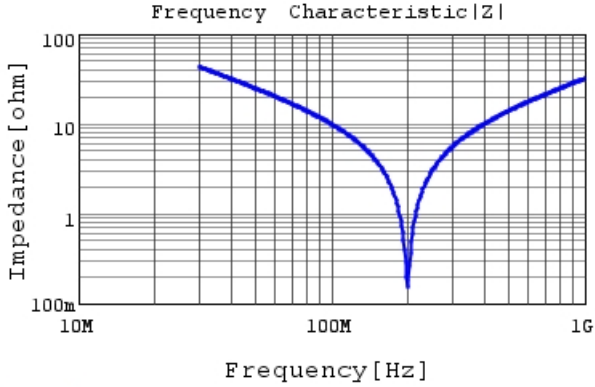
RDE5C2J121J1K1H03B |Z| DC0V, 25degC
