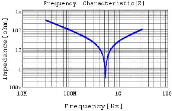
RDE5C2J180J1K1H03B |Z| DC0V, 25degC
