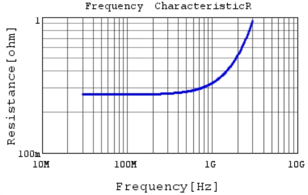
RDE5C2J180J1K1H03B R DC0V, 25degC
