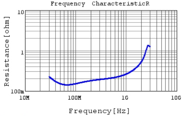
RDE5C2J560J1K1H03B R DC0V, 25degC
