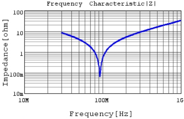
RDE5C2J561J1K1H03B |Z| DC0V, 25degC
