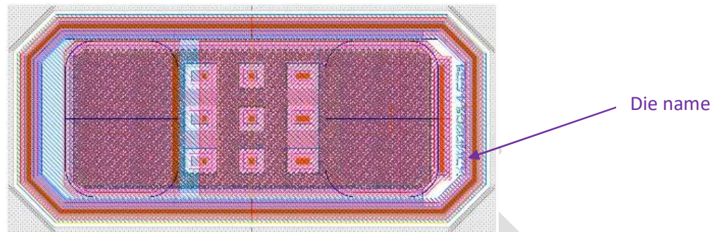
Figure 6 - Layout view
