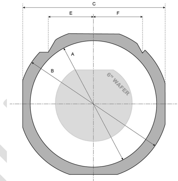
Figure 13 FF108 Frame with a 6" wafer
