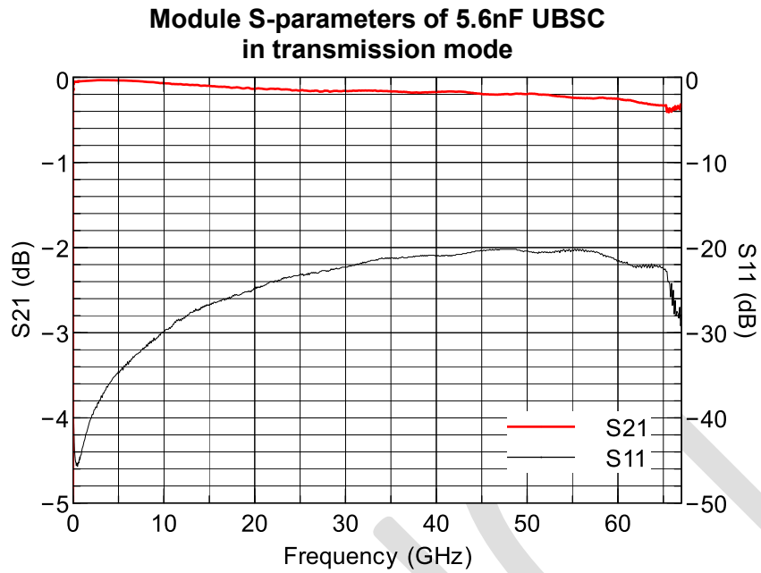
Figure 2 - 5.6nF UBSC simulated results (module of S-parameters)
