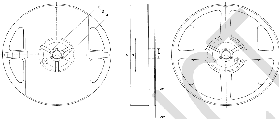
Figure 10 - Reel drawing
