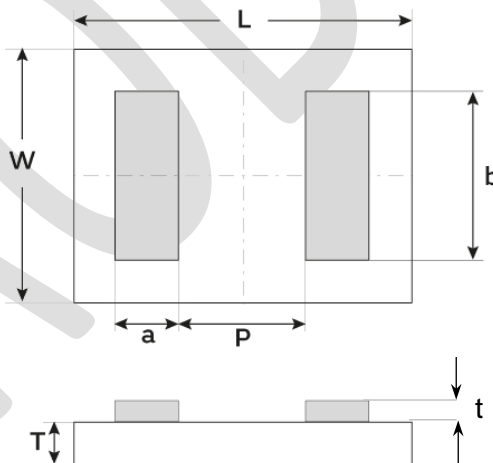
Figure 10 - Package outline drawing
