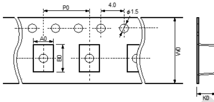
Figure 14 – Tape drawing (not to scale)
