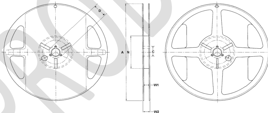
Figure 13 - Reel drawing
