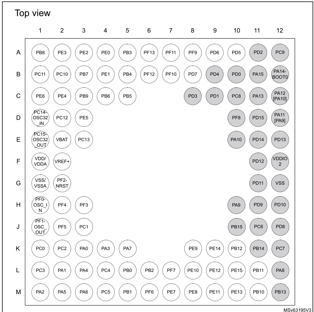
Figure 12. STM32G0B1Vxl UFBGA100 pinout
