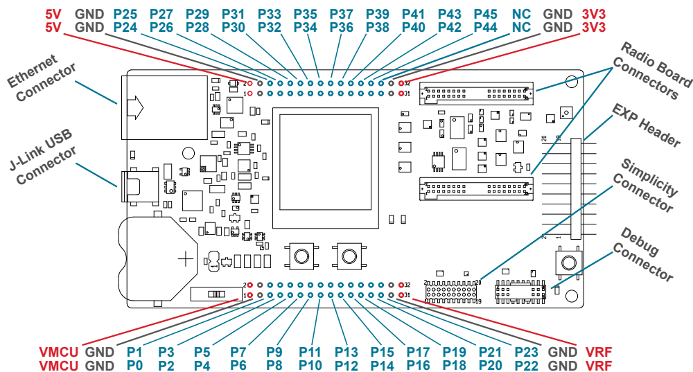
Figure 3.2. Wireless STK Mainboard (BRD4001A) Connector Layout
