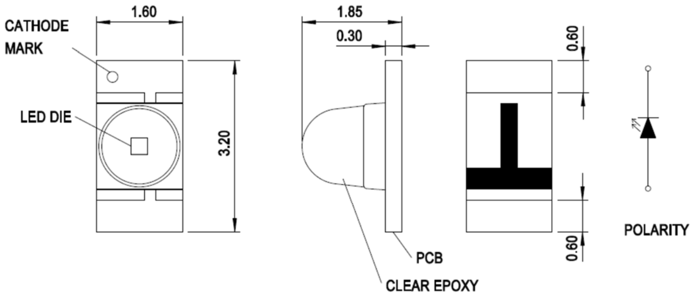
Figure 1: Package Dimensions
