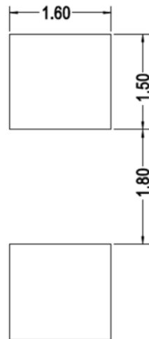
Figure 7: Recommended Soldering Land Pattern
