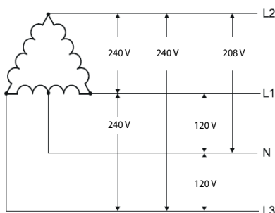
Fig. 4 Two-phase system with neutral (3-wire)
