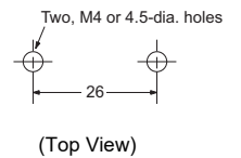
Mounting Hole Dimensions
