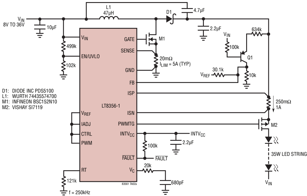
35W Buck-Boost-Mode LED Driver
