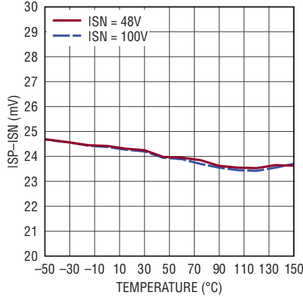
ISP-ISP Threshold at CTRL = 0.6V vs Temperature
