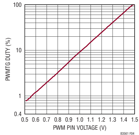
Figure 4. PWM Duty vs PWM Pin Voltages
