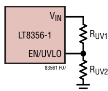
Figure 7. LT8356-1 Resistor Network for Accurate UVLO
