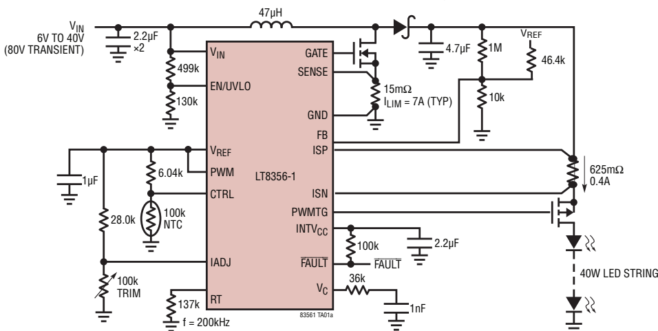
40W Boost LED Driver with Thermal Derating and Trim
