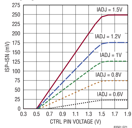
Figure 1. V_{ISP}-V_{ISN} vs CTRL and V_{IADJ} Pin Voltage
