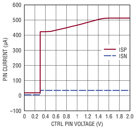
ISP/ISN Pin Current vs CTRL Voltage at ISP = 100V
