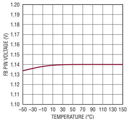
FB Open LED Threshold vs Temperature
