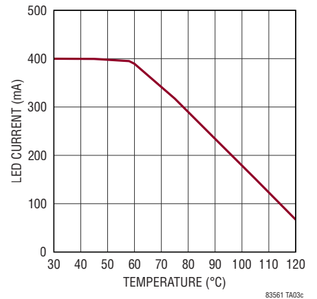
LED Current Thermal Derating
