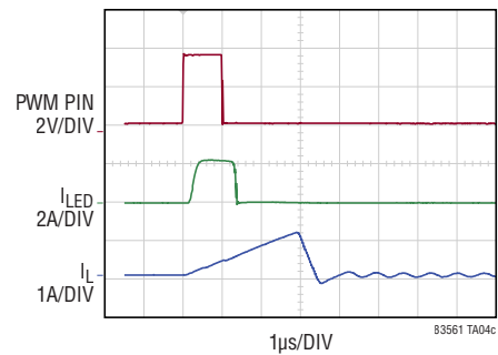
10,000:1 PWM Dimming at f_{PWM} = 100\text{Hz}
