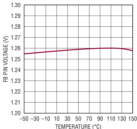
FB Overvoltage Threshold vs Temperature
