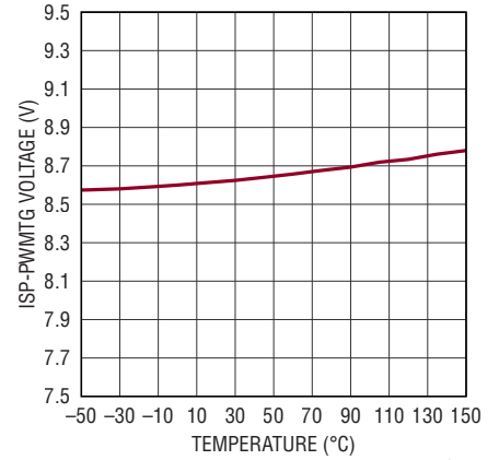
PWMTG ON Voltage vs Temperature
