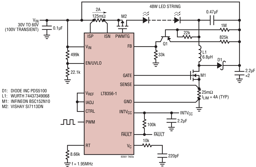
10,000:1 PWM Dimming at f_{PWM} = 100\text{Hz}
