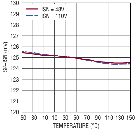
ISP-ISP Threshold at CTRL = 1V vs Temperature
