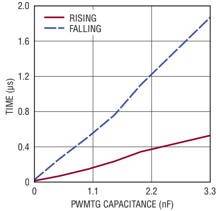
PWMTG Driver Rise/Fall Time vs PWMTG Capacitance
