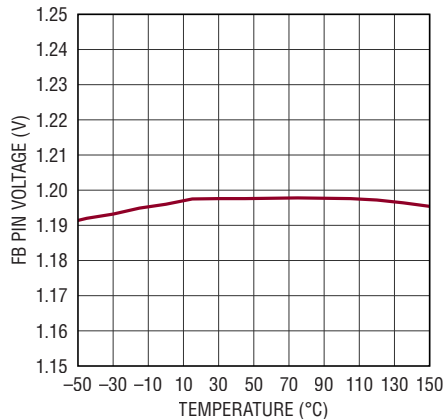
Output Voltage Regulation vs Temperature
