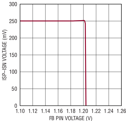
ISP-ISP Voltage vs FB Pin Voltage
