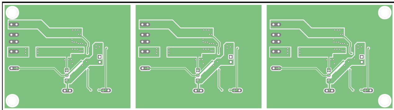
ADPL16000A/ADPL16000B/ADPL16000C EV Kits PCB Layout Diagram—Layer 2
