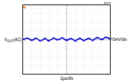
ADPL16000B OUTPUT VOLTAGE RIPPLE
