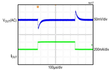
ADPL16000A LOAD TRANSIENT RESPONSE
