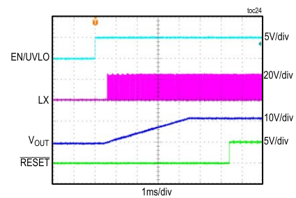
ADPL16000C STARTUP THROUGH ENABLE
