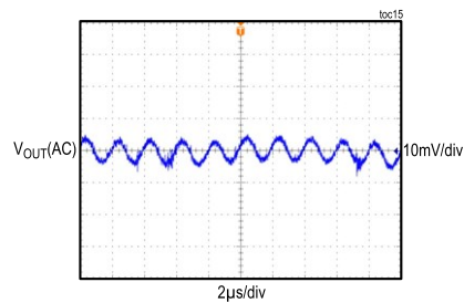
ADPL16000C OUTPUT VOLTAGE RIPPLE
