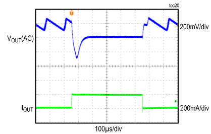
ADPL16000C LOAD TRANSIENT RESPONSE
