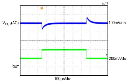
ADPL16000B LOAD TRANSIENT RESPONSE
