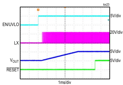
ADPL16000B STARTUP THROUGH ENABLE
