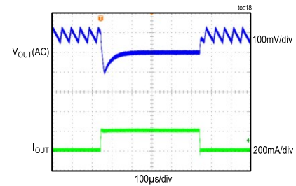
ADPL16000B LOAD TRANSIENT RESPONSE
