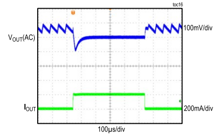
ADPL16000A LOAD TRANSIENT RESPONSE
