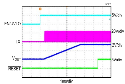
ADPL16000A STARTUP THROUGH ENABLE
