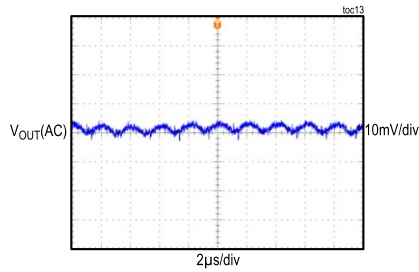
ADPL16000A OUTPUT VOLTAGE RIPPLE
