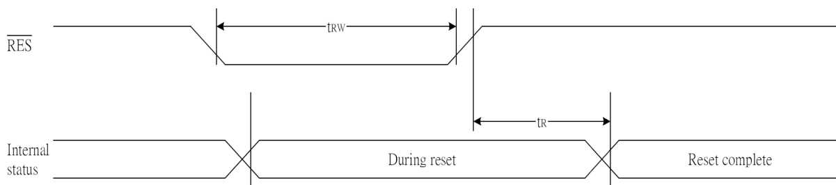
Figure 6: Reset Timing
