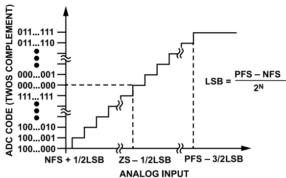
Figure 49. AD4857 Ideal Bipolar Input Transfer Function, N = 16 Bits
