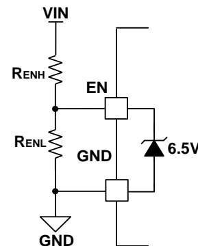
Figure 7: Programmable UVLO through EN
