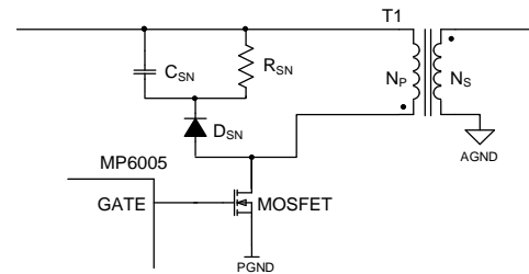
Figure 10: RCD Snubber
