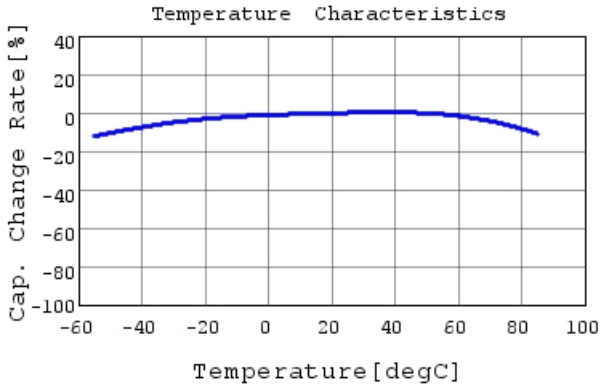
GRM188R60J226MEA0 C-Temp. capchange, DCO.0V,
