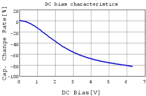
GRM188R60J226MEA0 C-DC bias capchange, 25.0c
