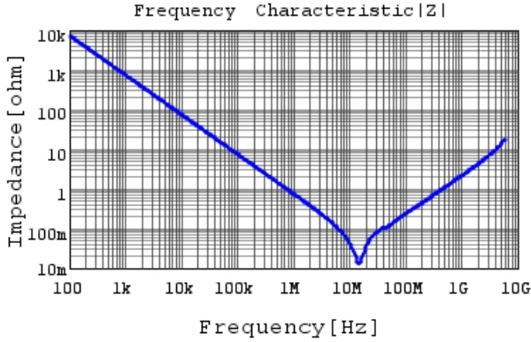
GCM188R71H224KA64 |Z| DCOV, 25degC
