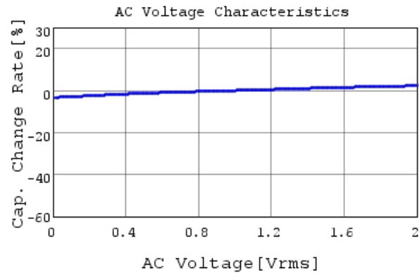
GCM188R71H224KA64 C-AC Voltage capchange, Dc
