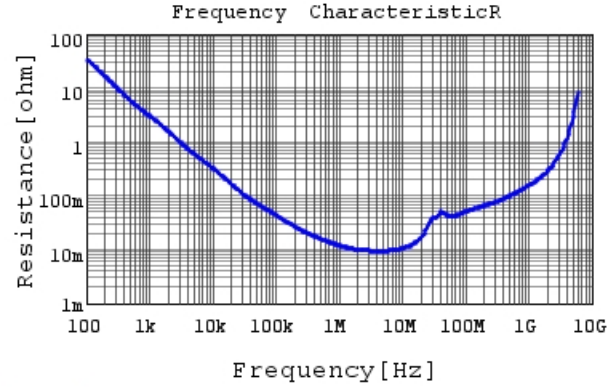
GCM188R71H224KA64 R DCOV, 25degC
