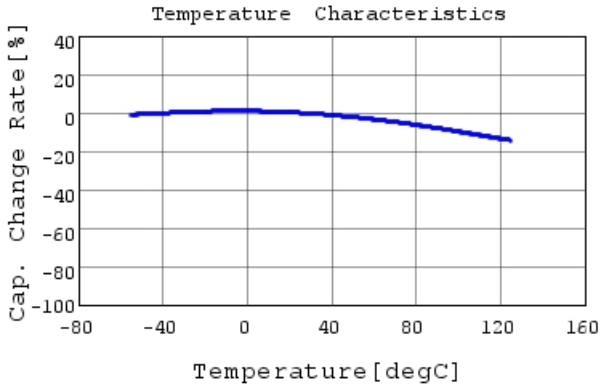
GCM188R71H224KA64 C-Temp. capchange, DC0.0V,
