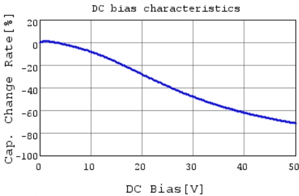
GCM188R71H224KA64 C-DC bias capchange, 25.0c
