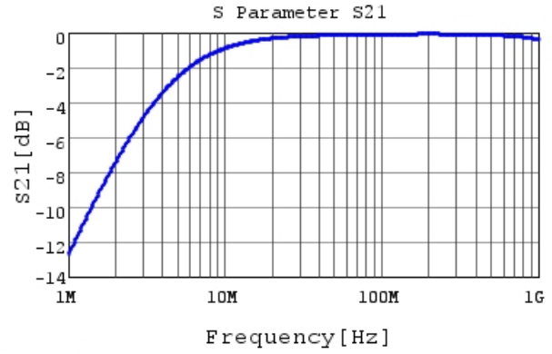
DK1B3EA471K86HAH01 S21 DCOV, 20degC
