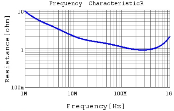
DK1B3EA471K86HBH01 R DCOV, 20degC
