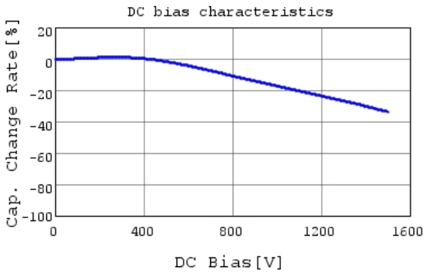
DK1B3EA471K86HBH01 C-DC bias capchange, 20.0
