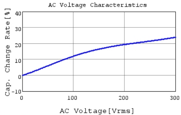
DK1B3EA471K86HBH01 C-AC Voltage capchange, I
