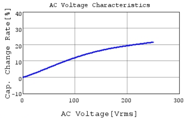
DK1B3EA681K86HAH01 C-AC Voltage capchange, I
