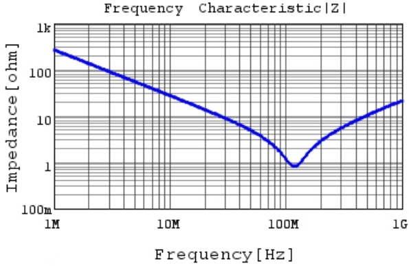
DK1B3EA681K86HAH01 |Z| DCOV, 20degC
