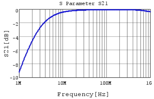
DK1B3EA681K86HAH01 S21 DCOV, 20degC
