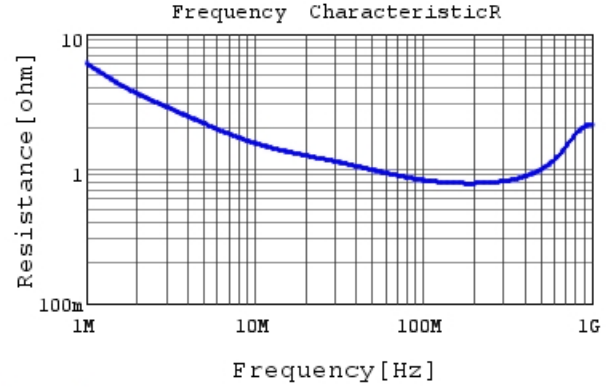
DK1B3EA681K86HAH01 R DCOV, 20degC
