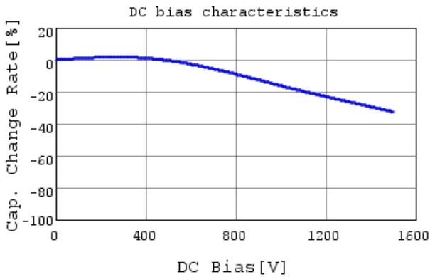
DK1B3EA681K86HAH01 C-DC bias capchange, 20.0
