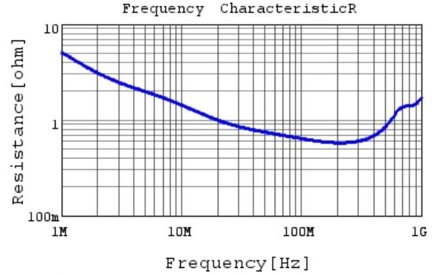
DK1E3EA102M86HAH01 R DCOV, 20degC
