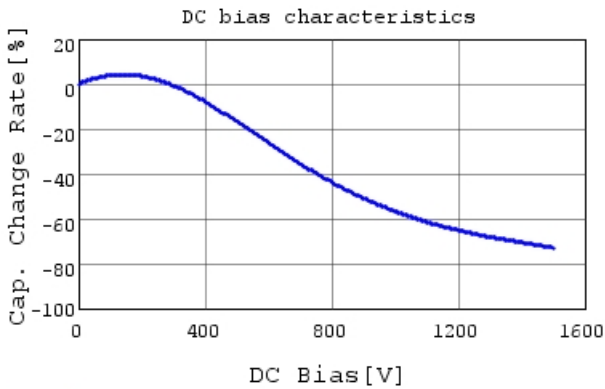
DK1E3EA102M86HAH01 C-DC bias capchange, 20.0
