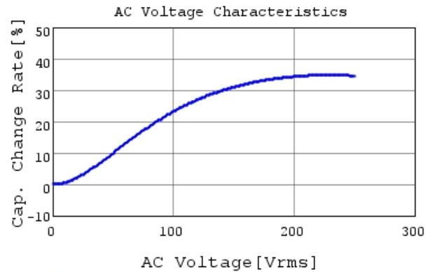
DK1E3EA102M86HAH01 C-AC Voltage capchange, I
