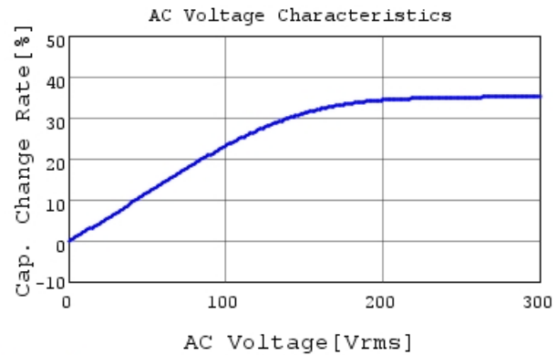
DK1E3EA152M86HBH01 C-AC Voltage capchange, I
