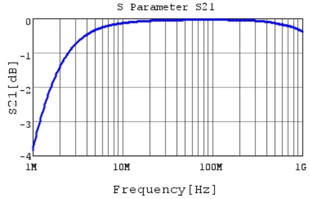
DK1E3EA152M86HBH01 S21 DCOV, 20degC
