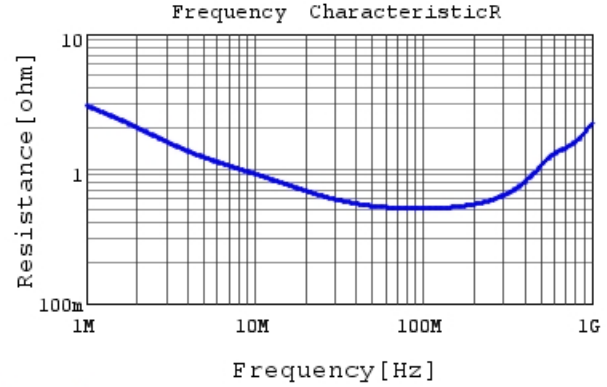
DK1E3EA152M86HBH01 R DCOV, 20degC
