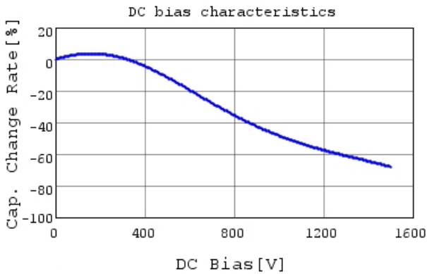
DK1E3EA152M86HBH01 C-DC bias capchange, 20.0
