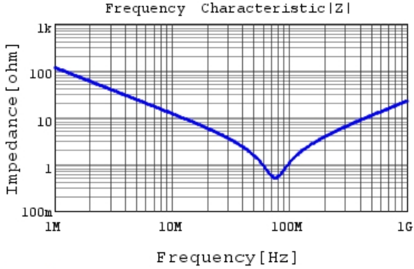
DK1E3EA152M86HBH01 |Z| DCOV, 20degC
