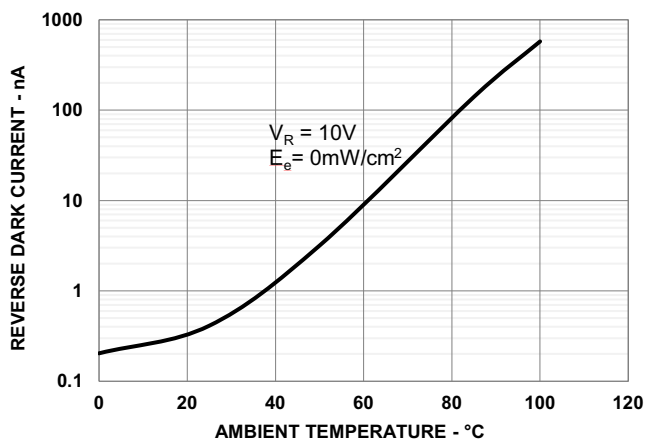
Figure 6: Reverse Dark Current vs Ambient Temperature
