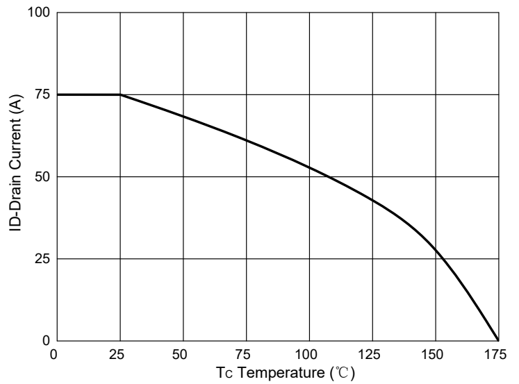
Fig. 10 - Drain Current
