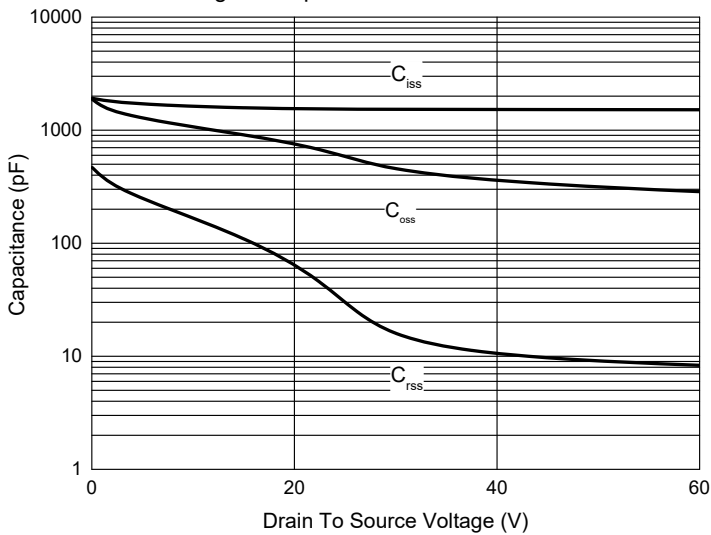
Fig. 5 - Capacitance Characteristics
