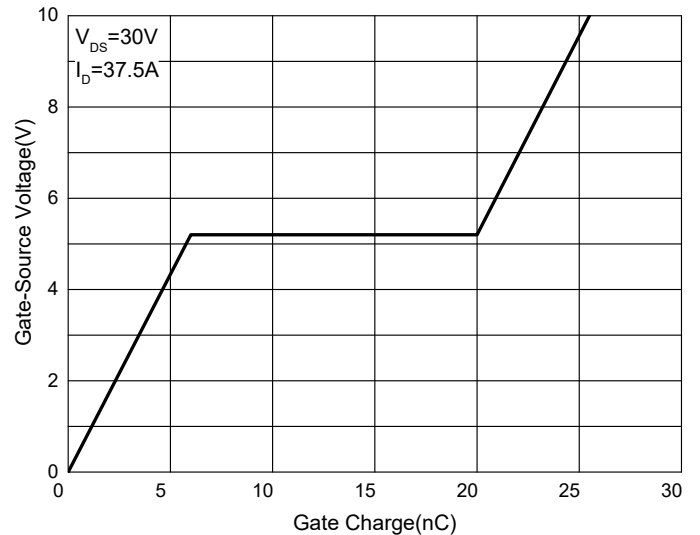
Fig. 6 - Gate Charge
