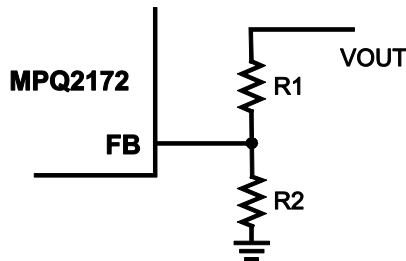
Figure 2: Feedback Network
