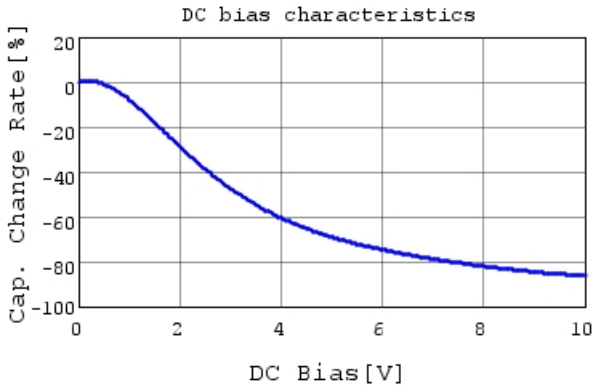
GRM21BR61A476ME15 C-DC bias capchange, 25.0c
