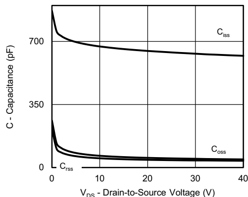
Capacitance
