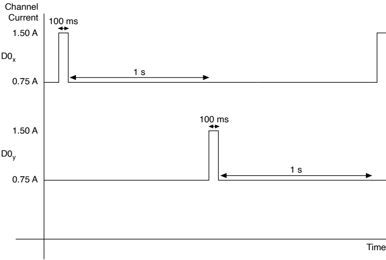
Figure 1. Short-circuit Behavior
