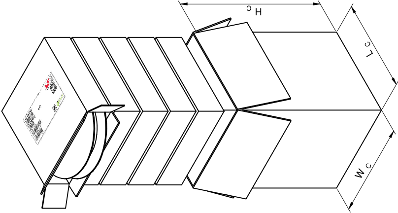
Packaging Specification - Outer Carton: [mm]
