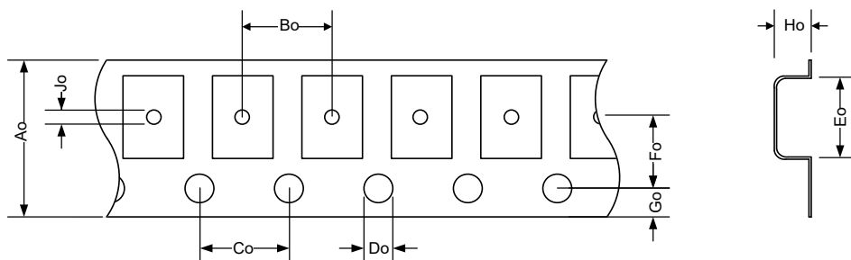
Figure 6: Tape information (drawing not to scale)
