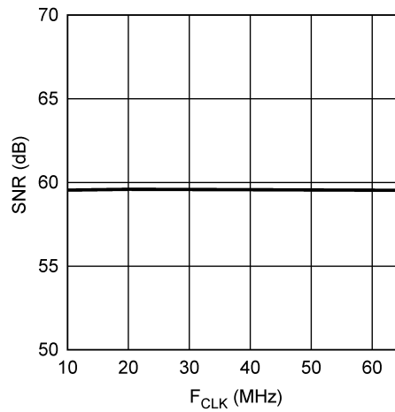
SNR vs. f_{CLK}
