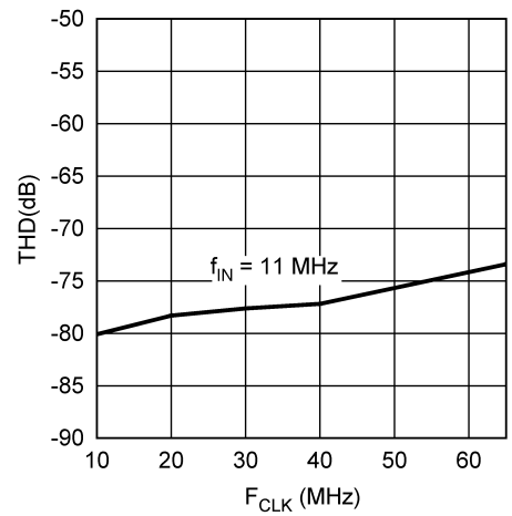
THD vs. f_{CLK}
