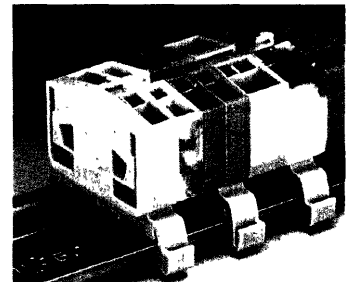
Terminal block strips with snap-in mounting feet on carrier rail TS 35
