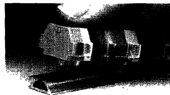
Terminal block strips with snap-in mounting feet on special aluminium carrier rail
