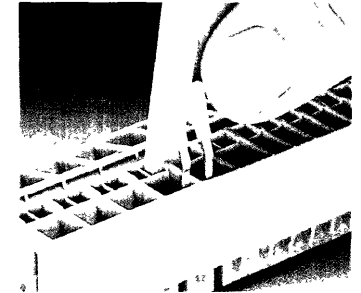
Commoning with comb-type jumper bar
