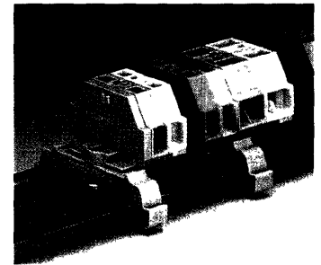
Terminal block strips with fixing flanges on carrier rail TS 35
