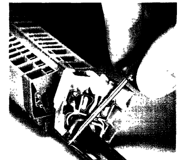
Removal of a ground (earth) conductor terminal block from the carrier rail
