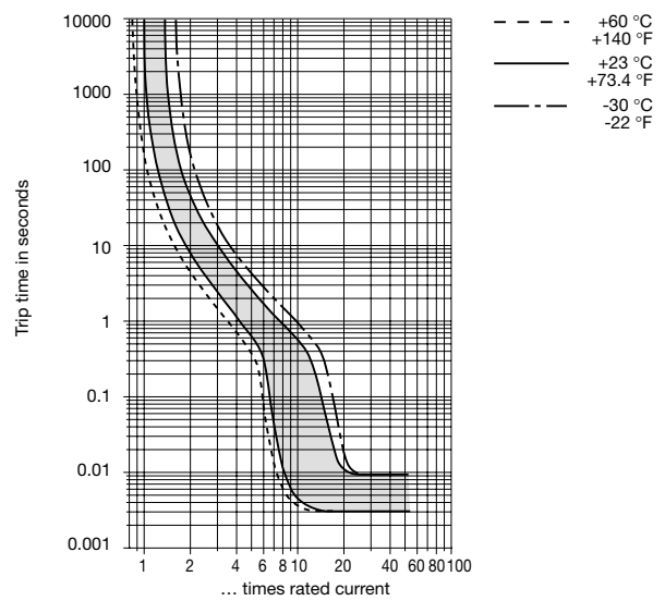
Type 3400 8 ... 16 A AC/DC 1)
