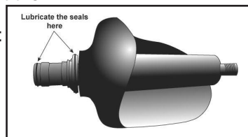
Diagram 2 Seal Lubrication
