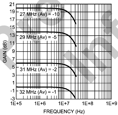
Gain vs Frequency R_F = 3k\Omega, V_S = \pm 15V
