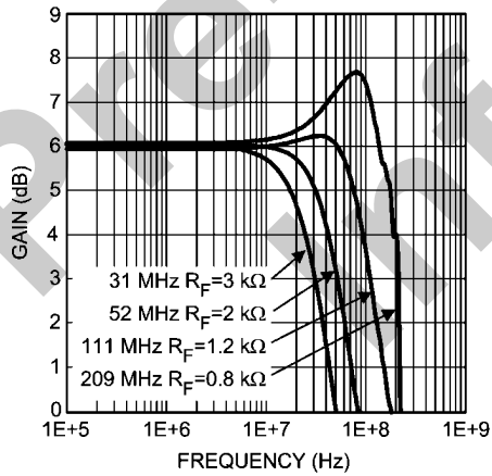
Gain vs Frequency V_S = \pm 15V, G = -2
