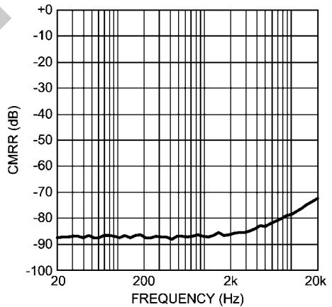
CMRR vs Frequency V_S = \pm 15V
