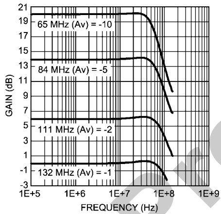
Gain vs Frequency R_F = 1.2k\Omega, V_S = \pm 15V
