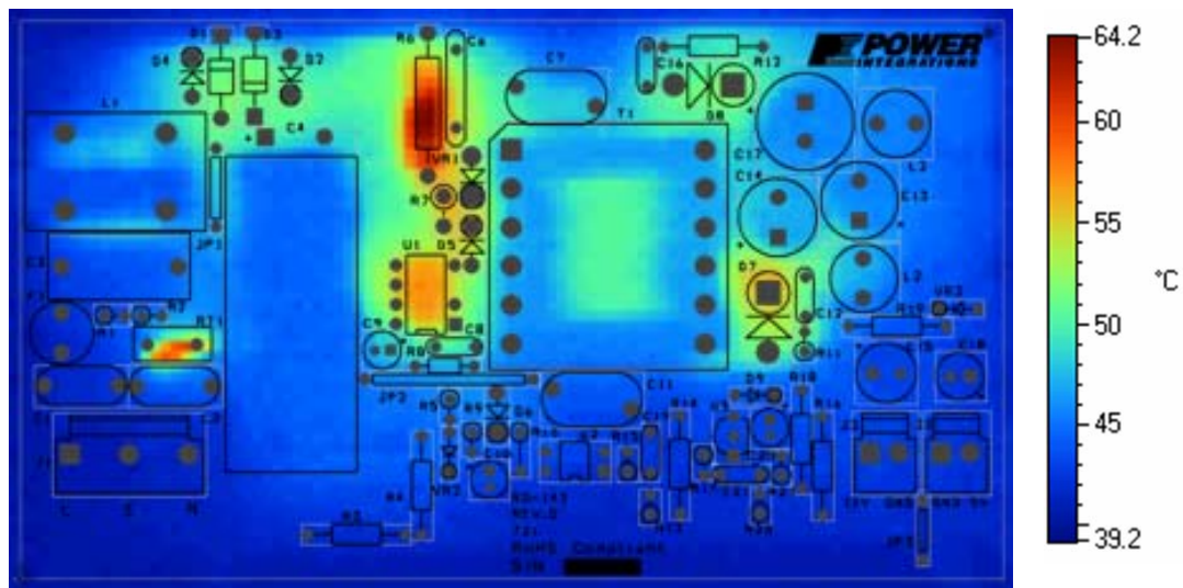
90 VAC, 35 W load, 21°C Ambient
