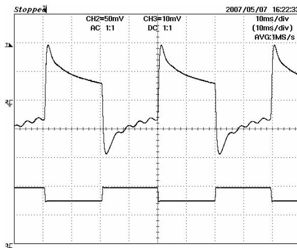
Figure 23 – 12 Volt output in response to 5 V transient, 265 VAC, 75-100-75% Load Step Output Voltage 50 mV/div, Output Current 1 A / div, 10 ms / div.
