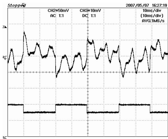
Figure 22 –12 Volt output in response to 5 V transient, 90 VAC, 75-100-75% Load Step Output Voltage 50 mV/div, Output Current 1 A / div, 10 ms / div.
