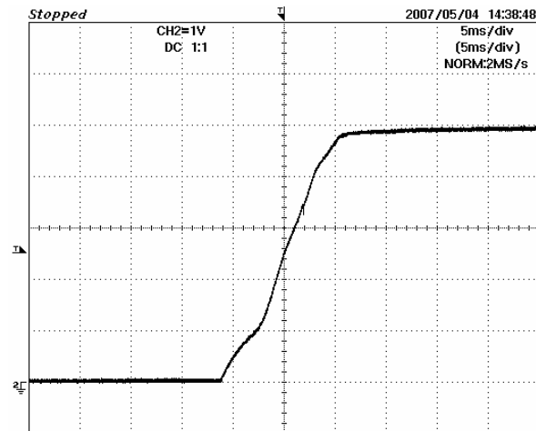
Figure 15 – 5 Volt Start-up Profile, Full load; 265 VAC; 1 V/div, 5 ms / div.
