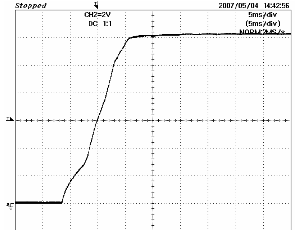
Figure 17 – 12 Volt Start-up Profile, Full load; 265 VAC; 2 V/div, 5 ms / div.
