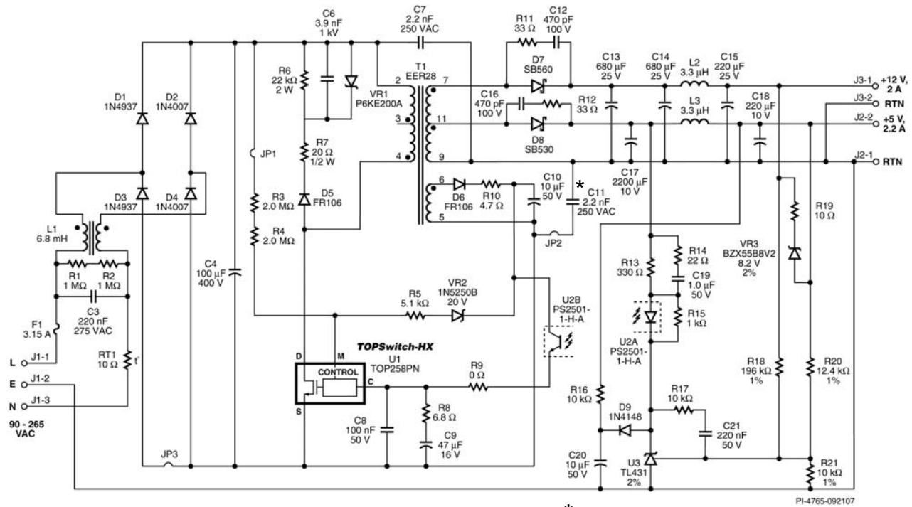
Figure 2 – Schematic.
