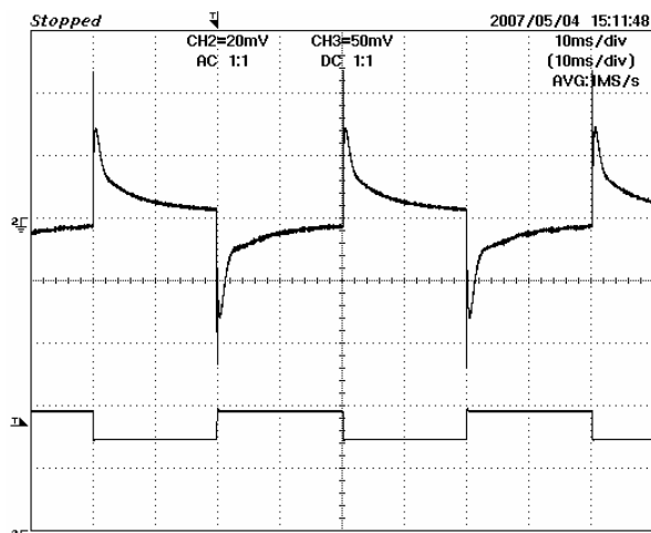
Figure 21 – 5 Volt Transient Response, 265 VAC, 75-100-75% Load Step Output Voltage 20 mV/div, Output Current 1 A / div, 10 ms / div.
