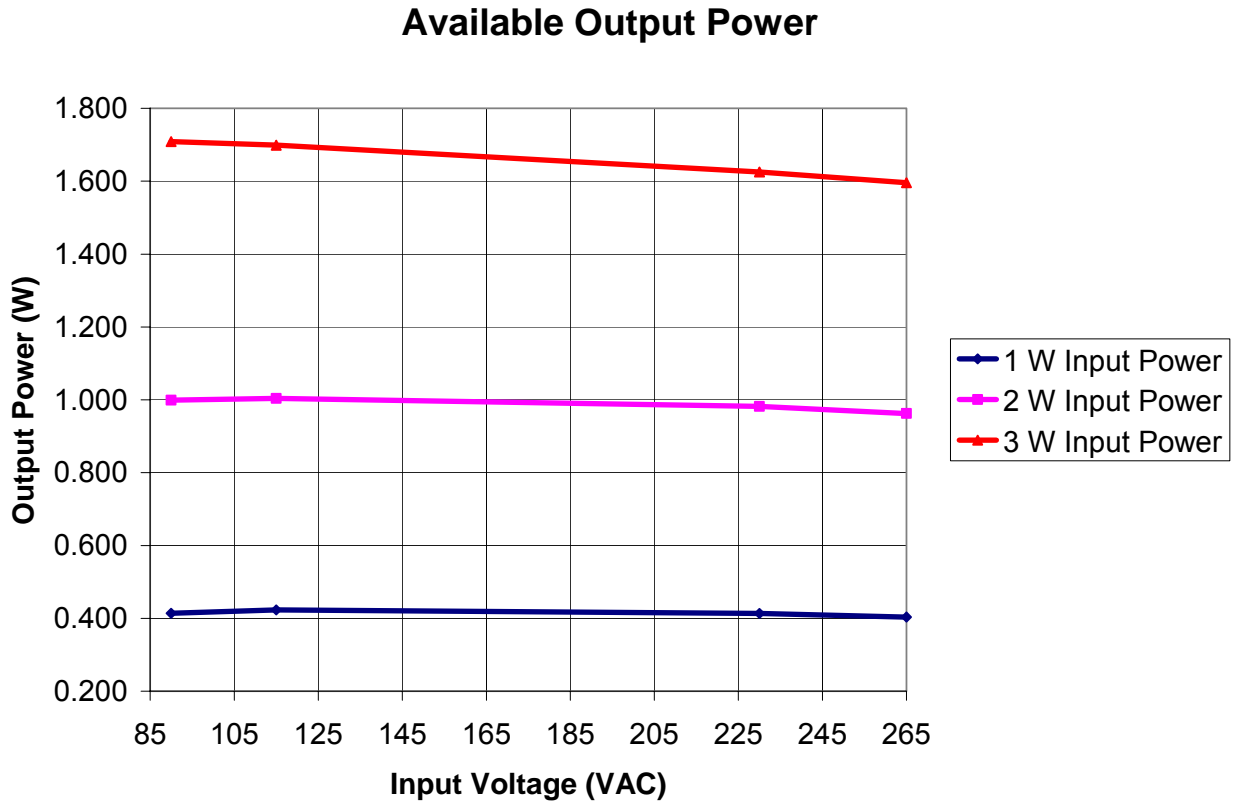
Figure 8 – Available Standby Output Power for Fixed Levels of Input Power
