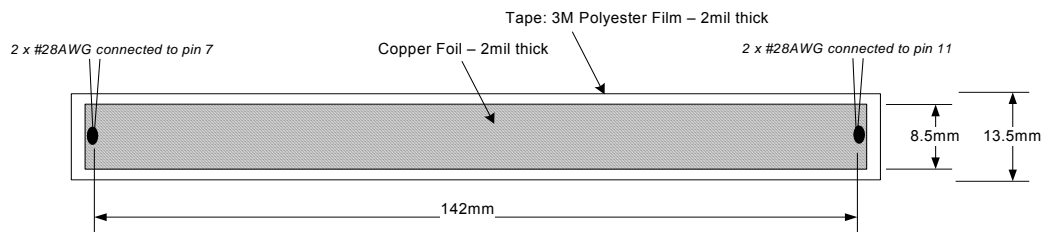
Figure 5 – Transformer Build Diagram.
