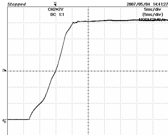
Figure 16 – 12 Volt Start-up Profile, Full load; 90 VAC; 2 V/div, 5 ms / div
