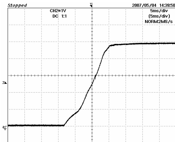
Figure 14 – 5 Volt Start-up Profile, Full load; 90 VAC; 1 V/div, 5 ms / div.
