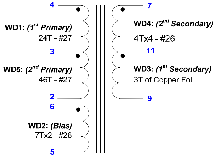
Figure 4 – Transformer Electrical Diagram.
