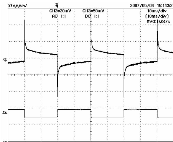
Figure 20 – 5 Volt Transient Response, 90 VAC, 75-100-75% Load Step. Output Voltage 20 mV/div, Output Current 1 A / div, 10 ms / div.
